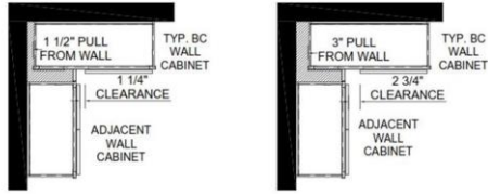
FIGURE 2 : TYPICAL INSTALLATION STANDARD OVERLAY
